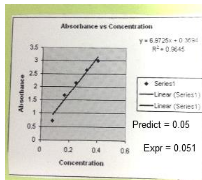
Beer's Law
