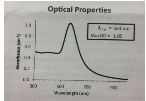
100 nm Gold Nanoparticle Standard
