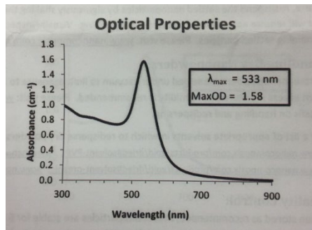
60 nm Gold Nanoparticle Standard
