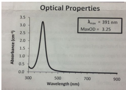
10 nm Silver Nanoparticle Standard
