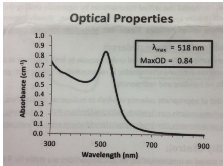
10 nm Gold Nanoparticle Standard
