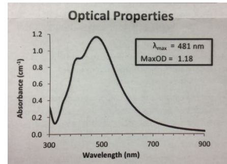
100 nm Silver Nanoparticle Standard
