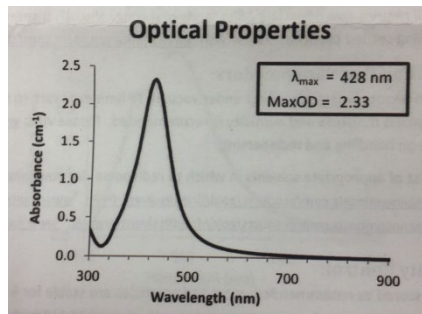
60 nm Silver Nanoparticle Standard
