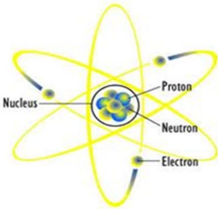
Atom
