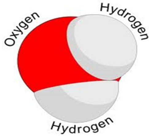
Water Molecule
