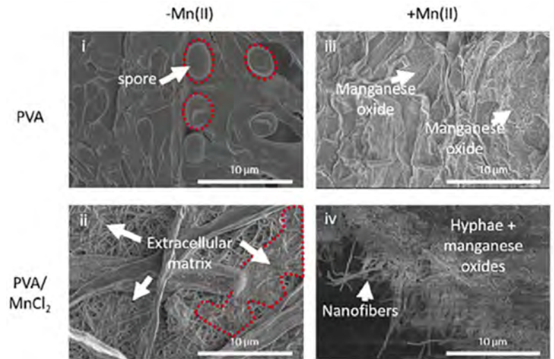
SEM images confirmed attachment of fungi to nanofibers i. Presence of spores indicated that nanofibers did not inhibit fungal reproduction iii. Coniothyrium sp. catalyzed the growth of sheet-like manganese oxide particles in Mn(II)-containing media ii., iv. Extracellular matrix appeared at the interface of nanofibers and hyphae (fungal cells)
