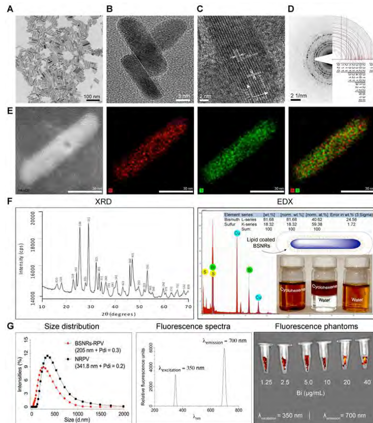
Synthesis and characterization of multimodal particles. TEM, EDX, XRD, size distribution and fluorescence.
