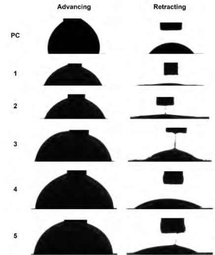
Above: Contact angle goniometer measurements (nano@stanford) of droplet spreading. Each polymer formulation showed better wetting than the Phos-Check (PC) control.
