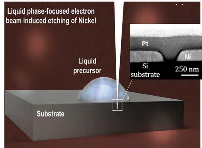
A focused electron beam penetrates through an aqueous sulfuric acid solution to induce etching of nickel. This technique permits nanoscale etching without damage to underlying materials. Inset: Cross-section of hole etched through a 170-nm thick Ni film.
