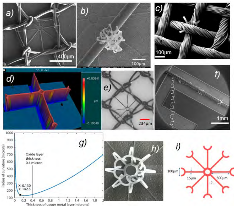
SEM images of Pop-up MEMS grippers transferred to a) Commercially produced Fabric Mesh b) Copper wire (diameter 78 \mu\text{m} ) c) Woven Polyester Fabric d) Zygo Surface Mapt-3D Model. e) Microscope image of pop-up gripper on Fabric Mesh f) Grippers integrated into serpentine structures released on to an elastic fiber. g) Graph-Radius of curvature of the gripper versus metal layer thickness. h) Pop-up gripper after release from the Si-Wafer. i) Gripper Design in L-Edit
