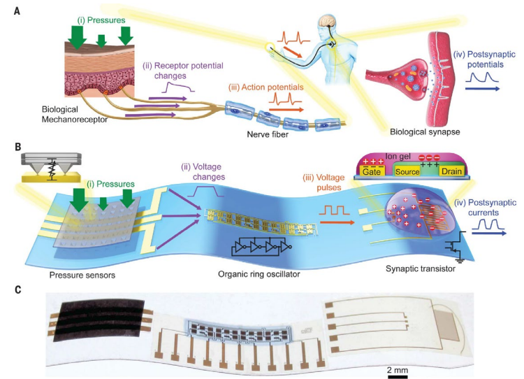
Figure: An artificial afferent nerve system in comparison with a biological one. (A) A biological afferent nerve that is stimulated by pressure. (B) An artificial afferent nerve made of pressure sensors, an organic ring oscillator, and a synaptic transistor. (C) A photograph of an artificial afferent nerve system.
