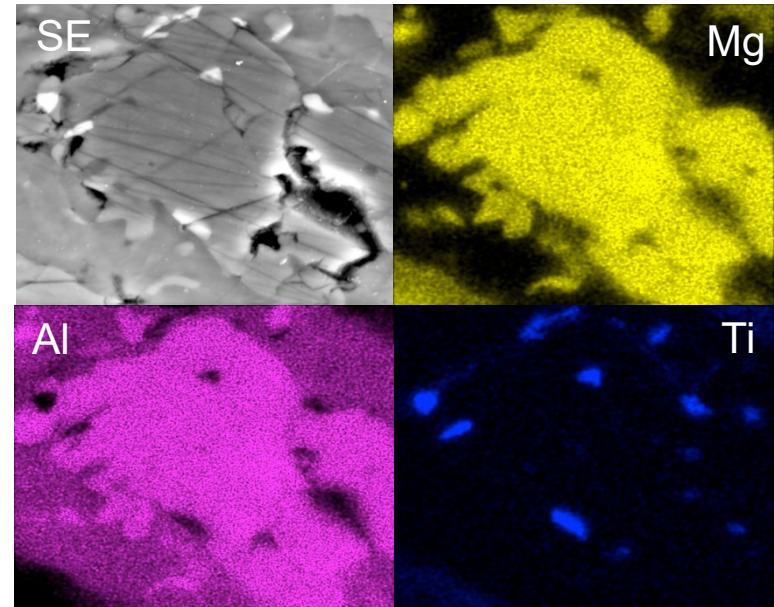
10 keV secondary electron image and EDX Mg, Al and Ti element maps showing Ti inclusions in the mineral spinel in the primitive chondritic meteorite Efremovka. FOV for each image is approximately 8 \mu\text{m} .
