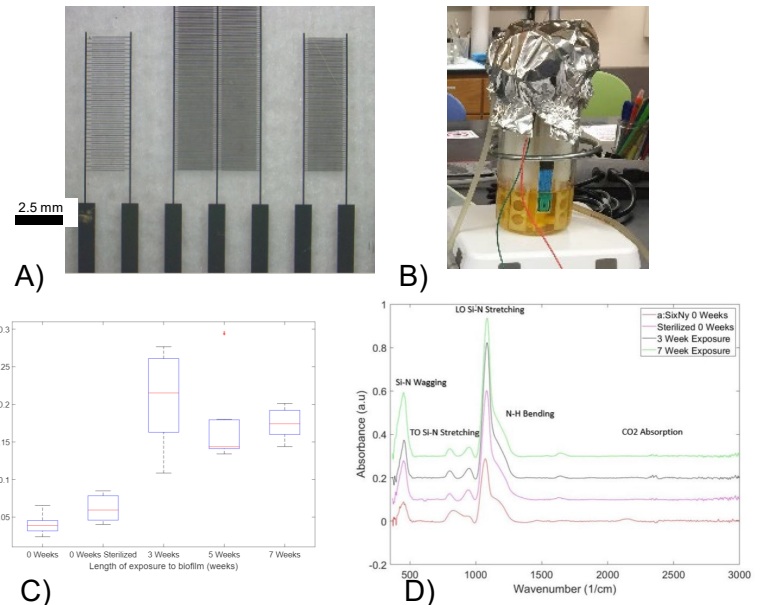
A) Micro-fabricated Impedance Spectroscopy sensor used to monitor biofilm growth (feature size: 30\ \mu\text{m} ). B) Biofilm reactor to control biofilm growth. C) Surface resistivity increase of Al due to prolonged biofilm exposure. D) FTIR of potential inert a\text{:Si}_x\text{N}_y\text{-H} encapsulation layer (no changes in vibration modes after biofilm exposure).
