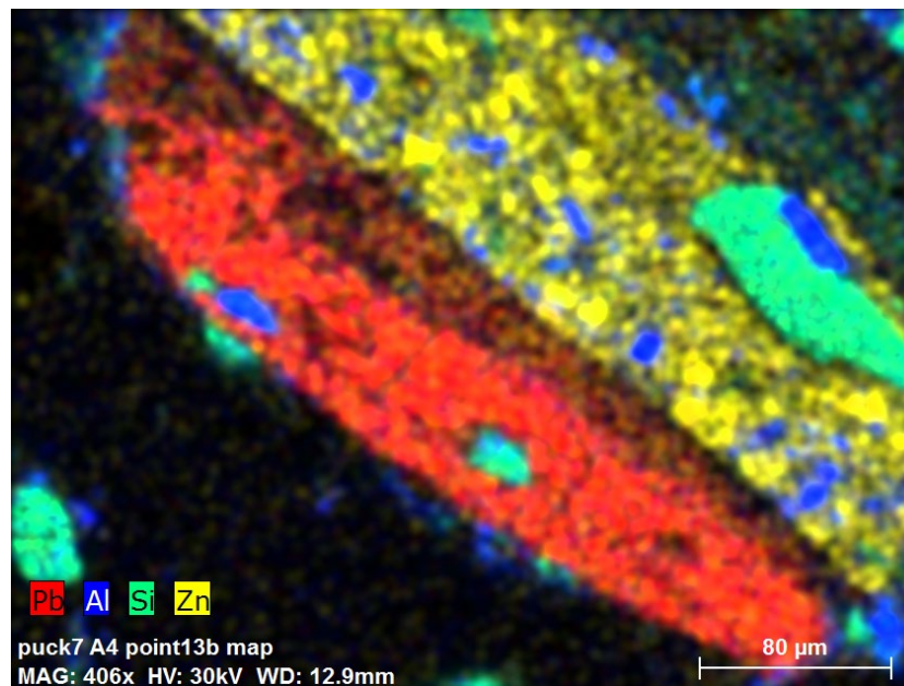
Lead contaminated soils identified using SEM / EDS for targeted precision FIB sectioning, were further analyzed with HRTEM, STEM / EDS mapping and electron diffraction
