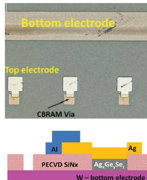
Top view and cross-section of PMC devices with access to bottom electrode, top electrode bond pad, and PMC/CBRAM via
