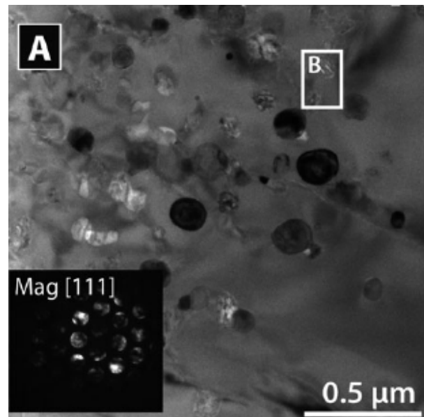
TEM bright-field images and SAED patterns of the biotite breakdown material along shock vein margins. The nanometer-sized dark inclusions in this image are Fe-rich
