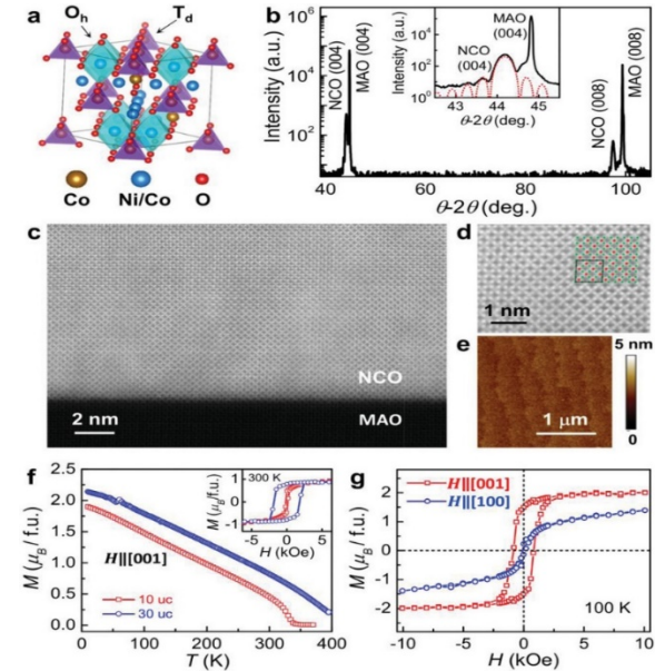
Characterizations of NCO films. a) Schematic crystal structure of NCO. b) XRD \theta - 2\theta scan c) HAADF-STEM image d) a higher-magnification image e) AFM topography image. f) Out-of-plane M vs T for 10 and 30 uc films. Inset: M vs H at 300 K. g) M vs H in out-of-plane and in-plane magnetic fields for the 10 uc film at 100 K.
